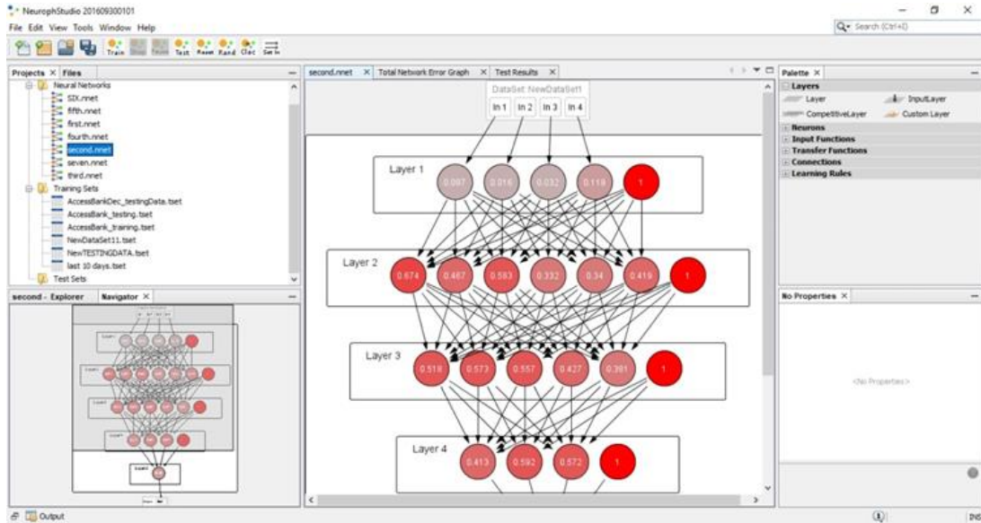
Fig. 1 Sample of One of the Trained Networks in NeurophStudio (Source: NeurophStudio 2.6).
